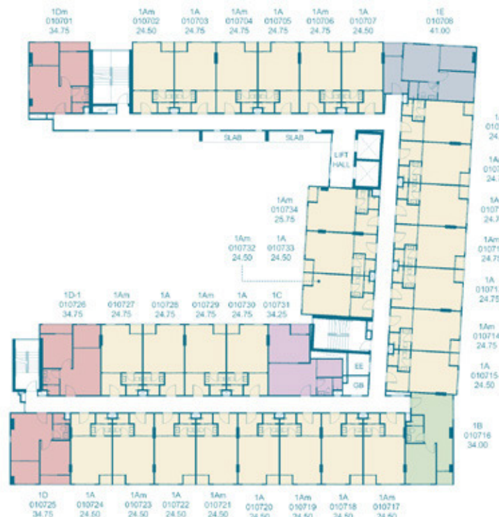
7 th FLOOR PLAN
